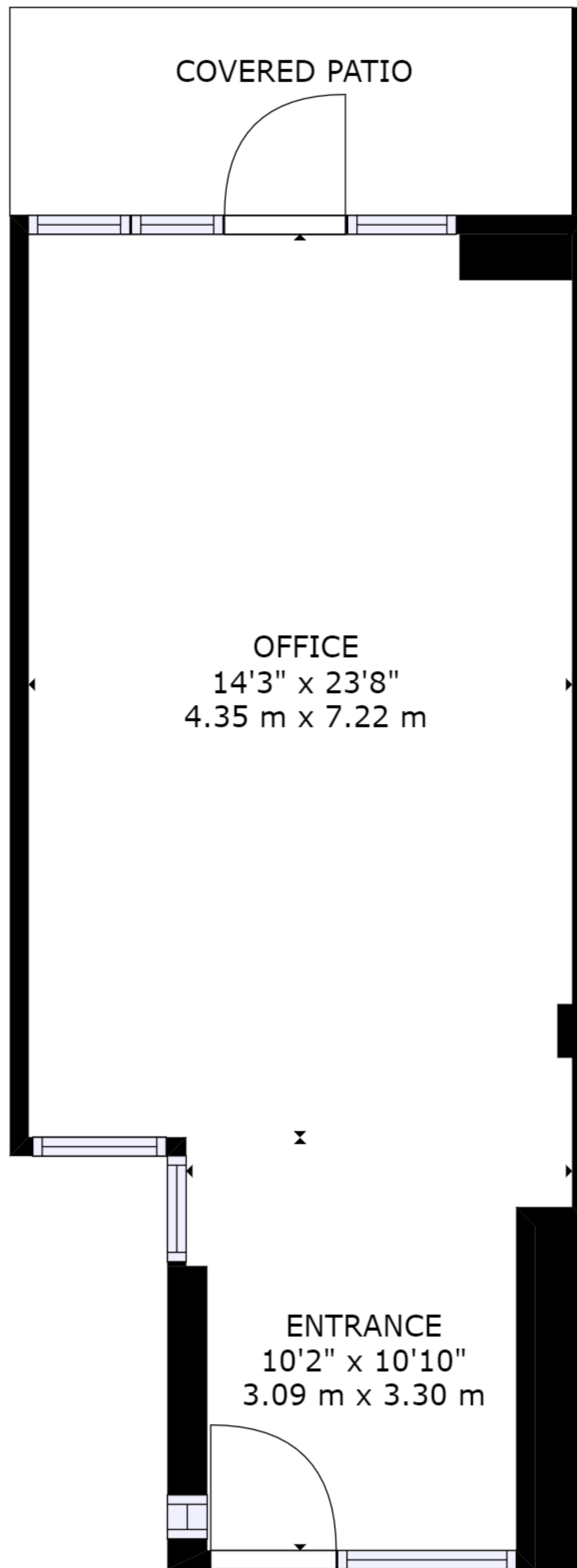
FLOOR 1
